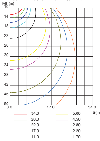
C0 PLANE ISOLUX DIAGRAM (UNIT:lx)
