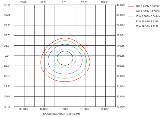
ISOLUX DIAGRAM
