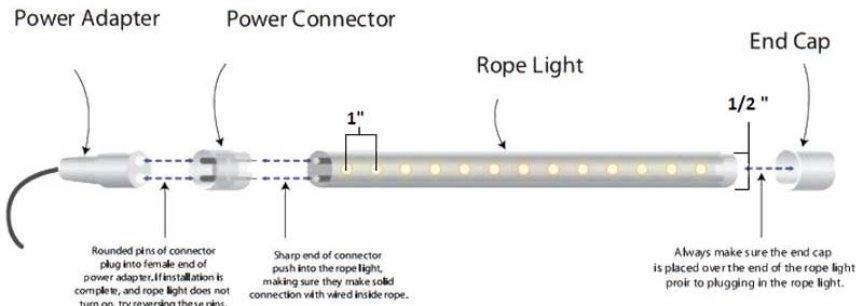
LED Rope Light Components
